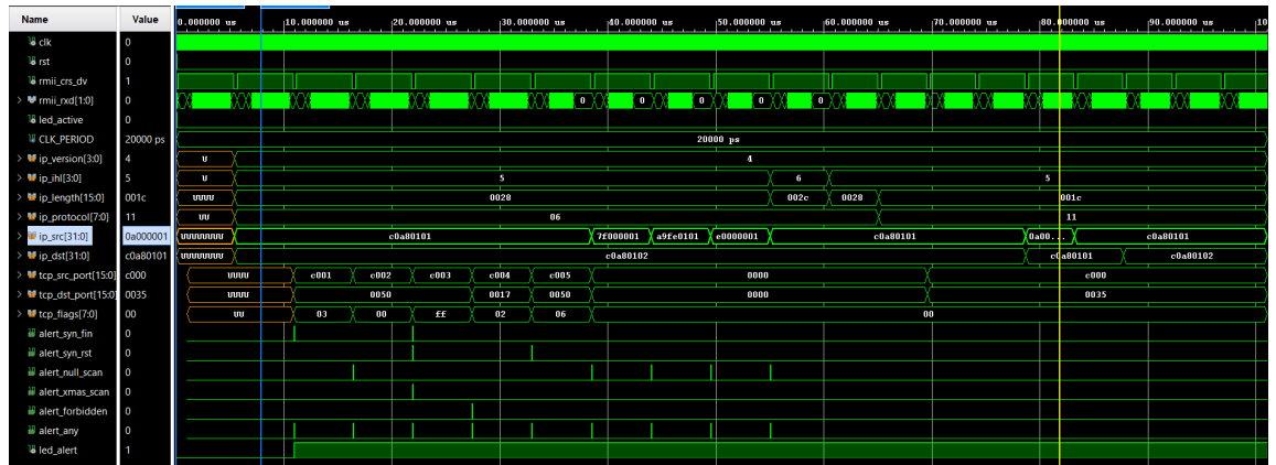
Figure 5.1: Simulation waveform showing TCP rules T1–T5 firing in sequence.
