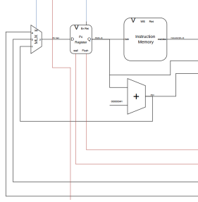
Figure 2.3: RV32ICore IF Stage
